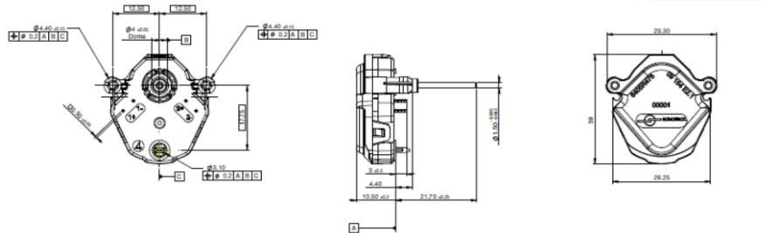
Reference for pins measurement
