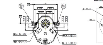
Reference for pins measurement
