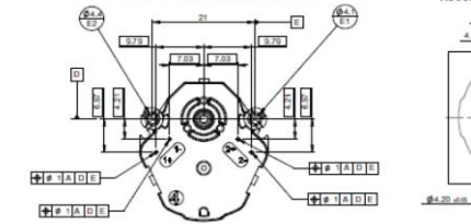
Reference for pins measurement
