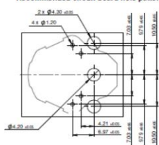
Recommended circuit board hole pattern
